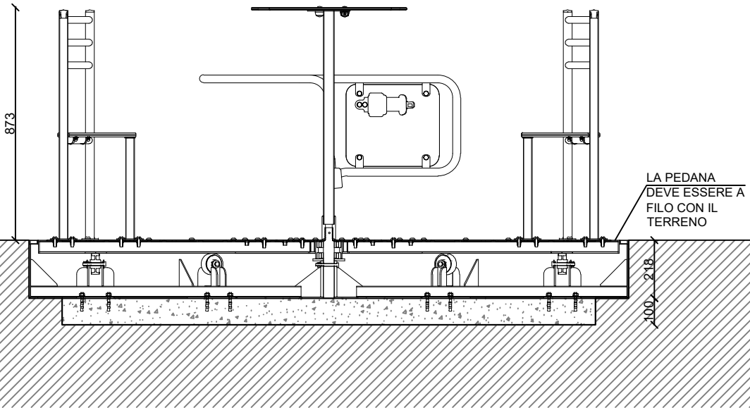
VISTA LATERALE (LATERAL VIEW)
